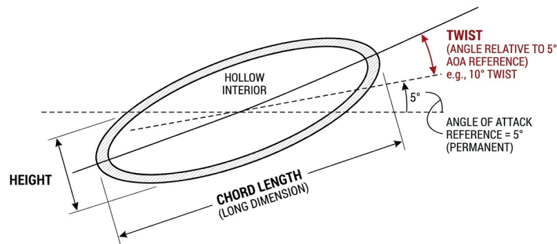
Figure 1: Cross-sectional view of the wing's airfoil. The height and chord lengths are measured from the outside edges of the airfoil.
